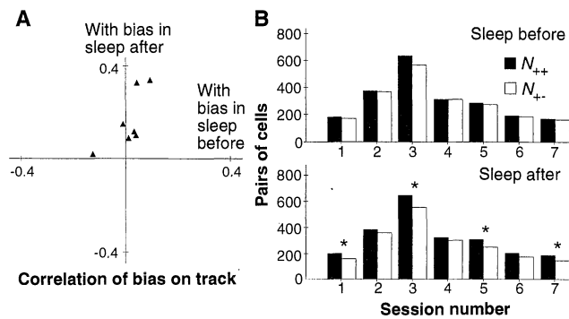
Fig. 2. Relation of temporal bias on the track with bias before and after track running. (A) Scatterplot of correlation coefficients for the seven recording sessions. Each correlation coefficient is calculated from a plot of the type in Fig. 1C. The horizontal coordinate of each point represents the overall correlation, for all pairs of cells from the recording session, between the temporal bias during track running and the temporal bias during the 15 min of sleep before the track-running session. The vertical coordinate represents the correlation of the bias during track running and the bias during sleep after the track-running session. (B) Histogram plots of N_{++} and N_{+-} , for each of the seven recording sessions, during periods of sleep before and after the track-running session. Asterisks mark sessions where N_{++} is significantly greater than N_{+-} ( P < 0.05 ).
